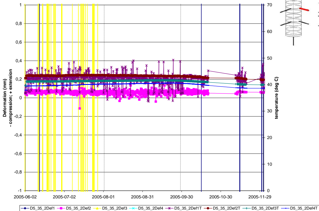
Deformation measurements Borehole D5:3.5(2)
