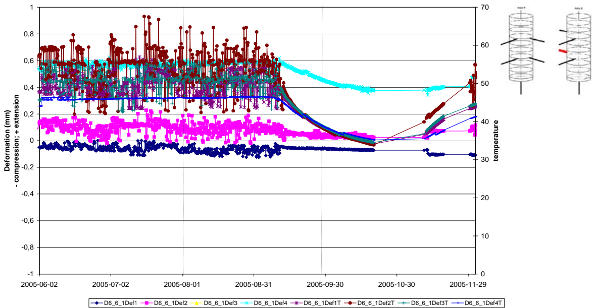
Deformation measurements Borehole D6:6(1)
