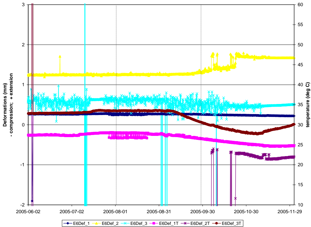
Vertical deformations adjacent to Deposition Hole 6 in borehole E6
