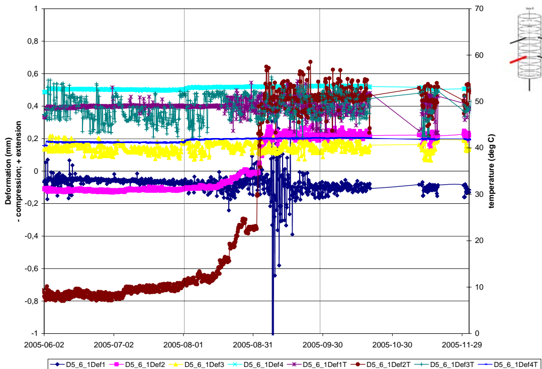
Deformation measurements Borehole D5:6(1)
