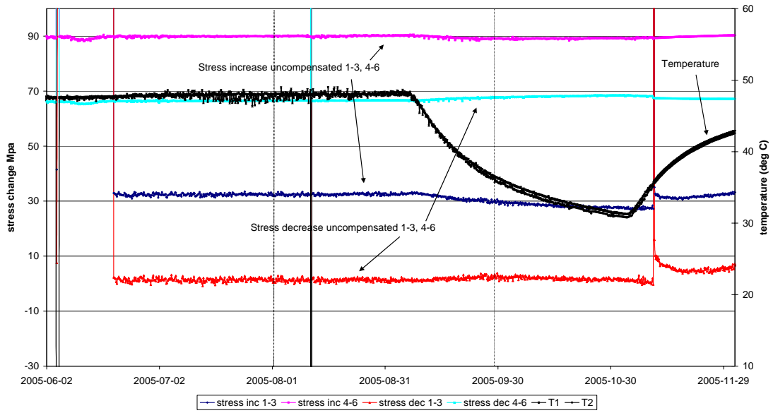
Biaxial stressmeter E6 Maximum stress increase and stress decrease in plane perpendicular to borehole axis
