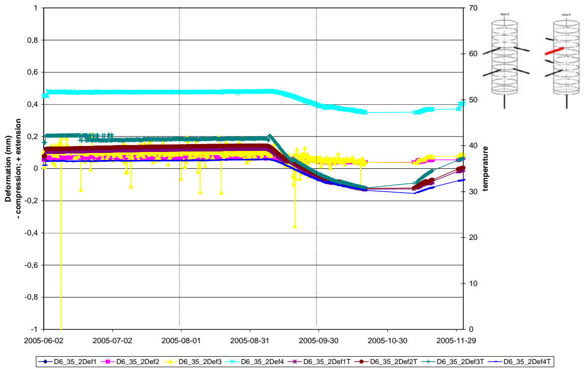
Deformation measurements Borehole D6:3.5(2)
