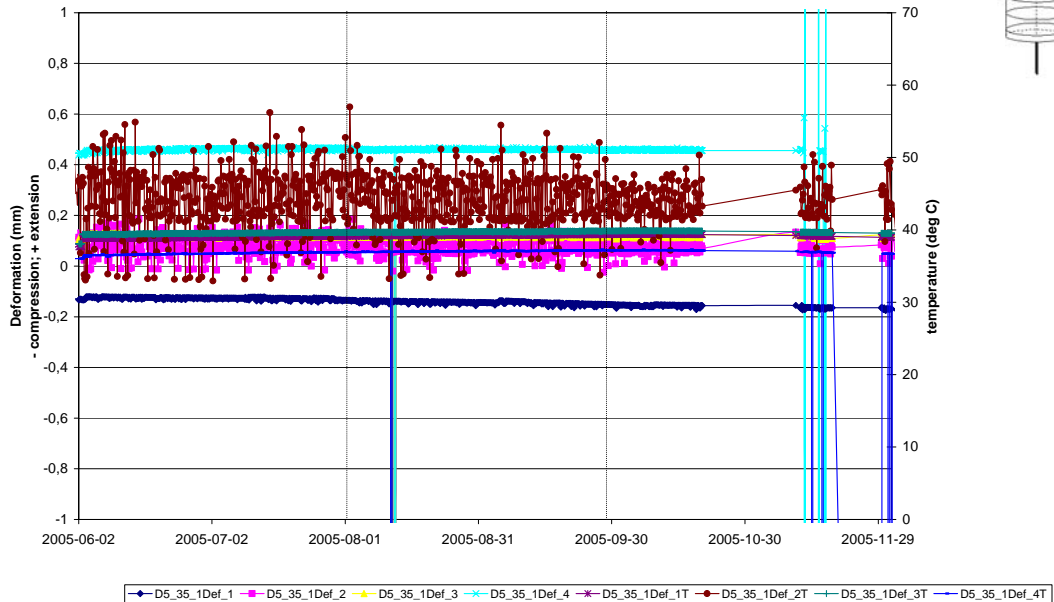
Deformation measurements Borehole D5:3.5(1)
